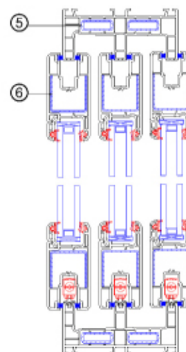
Vertical Assembly Drawing
