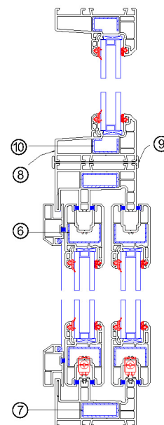
Vertical Assembly Drawing
