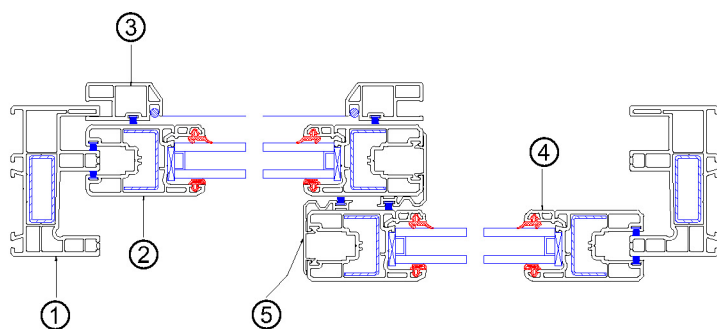
Horizontal Assembly Drawing
