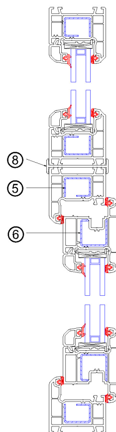
Vertical Assembly Drawing
