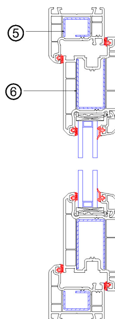
Vertical Assembly Drawing
