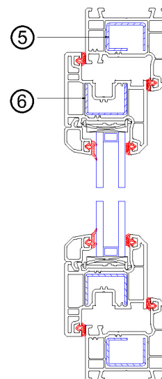
Vertical Assembly Drawing
