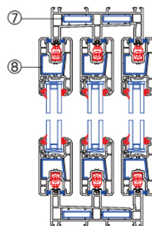
Vertical Assembly Drawing
