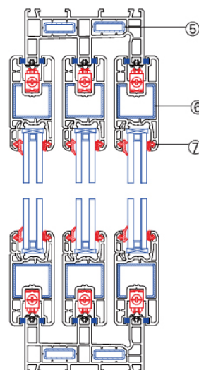
Vertical Assembly Drawing
