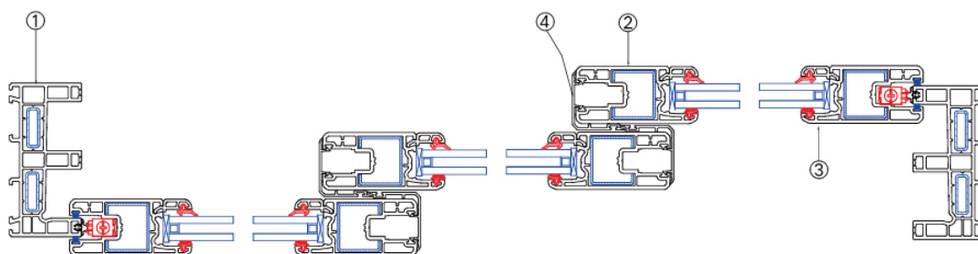
Horizontal Assembly Drawing
