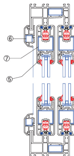
Vertical Assembly Drawing
