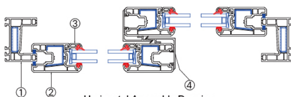
Horizontal Assembly Drawing
