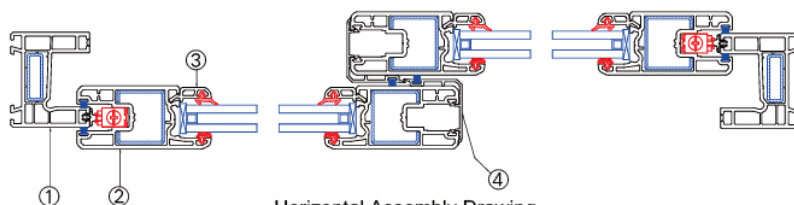
Horizontal Assembly Drawing
