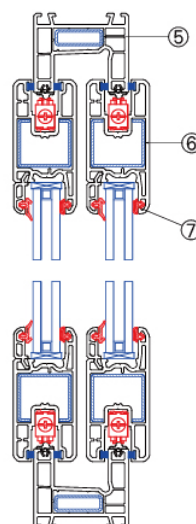
Vertical Assembly Drawing
