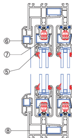
Vertical Assembly Drawing
