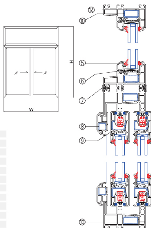
Vertical Assembly Drawing
