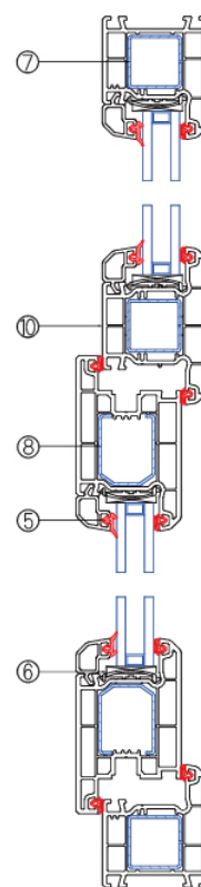
Vertical Assembly Drawing
