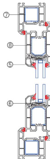
Vertical Assembly Drawing
