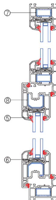
Vertical Assembly Drawing
