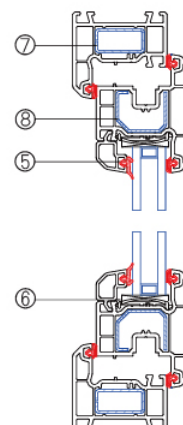
Vertical Assembly Drawing
