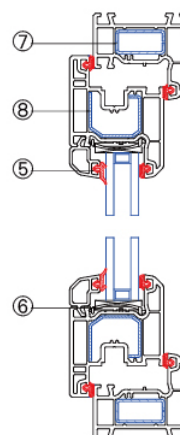
Vertical Assembly Drawing
