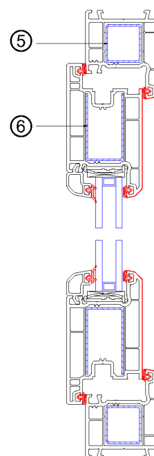
Vertical Assembly Drawing
