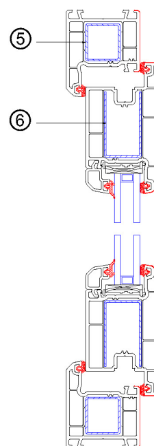
Vertical Assembly Drawing
