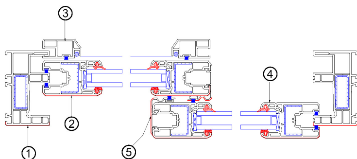
Horizontal Assembly Drawing
