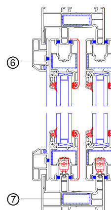
Vertical Assembly Drawing
