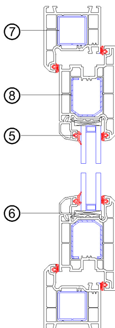
Vertical Layout Drawing
