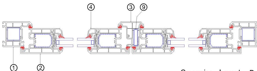
Crosswise Layout Drawing
