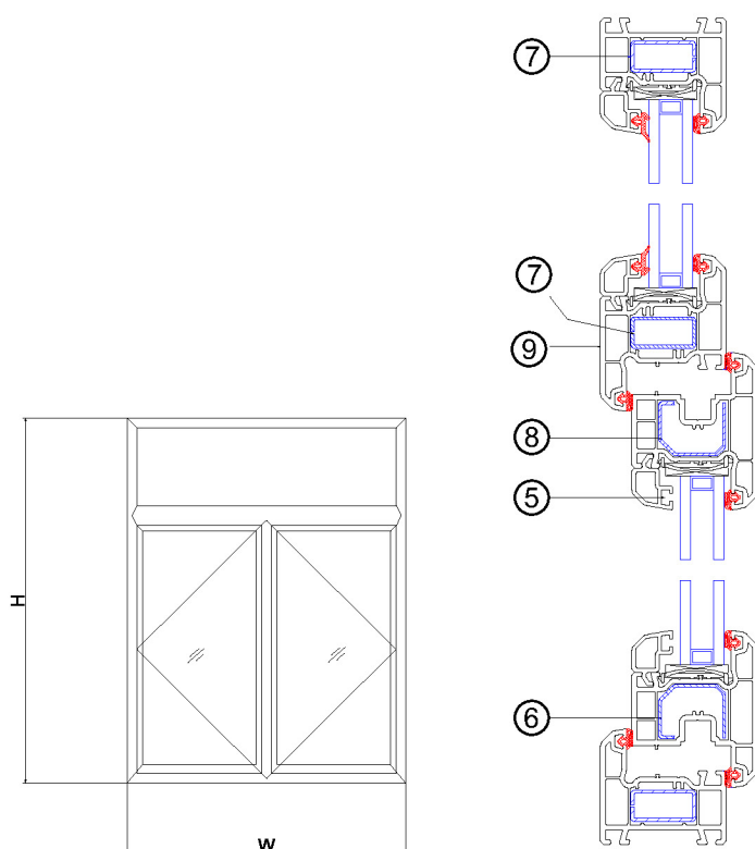
Vertical Layout Drawing
