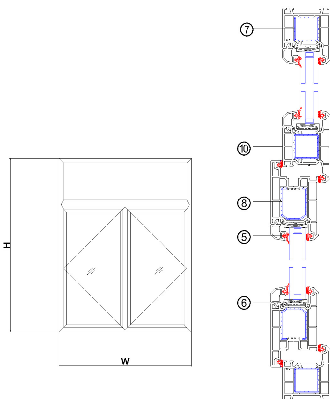
Vertical Layout Drawing
