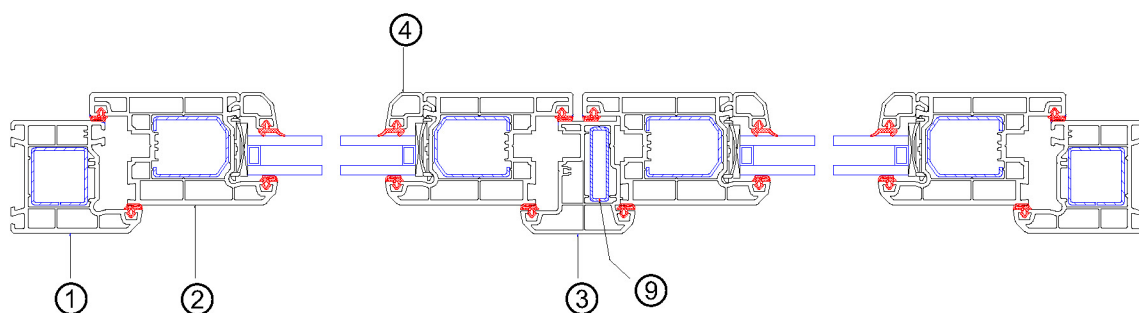
Crosswise Layout Drawing
