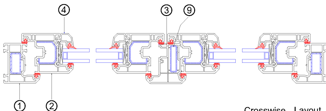
Crosswise Layout Drawing
