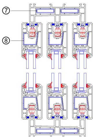
Vertical Layout Drawing
