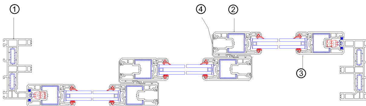
Crosswise Layout Drawing
