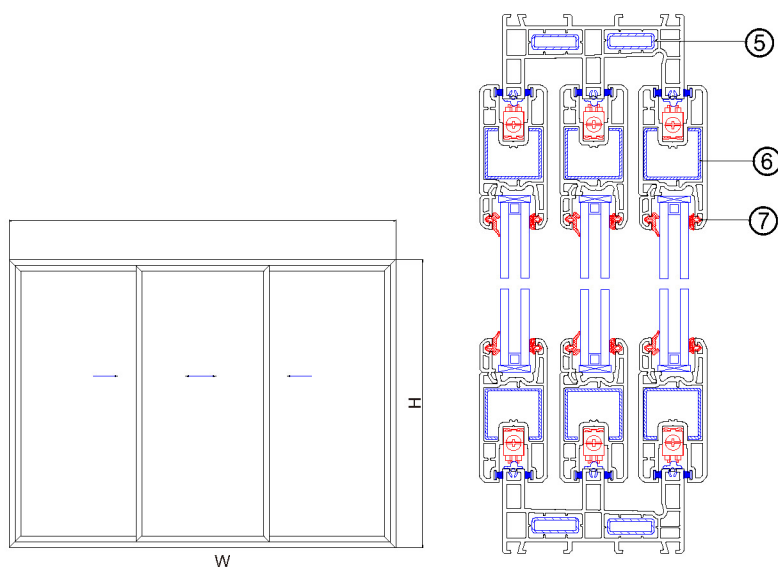
Vertical Layout Drawing
