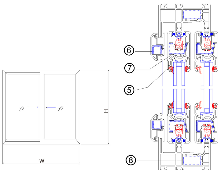
Vertical Layout Drawing
