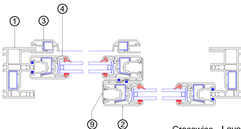
Crosswise Layout Drawing
