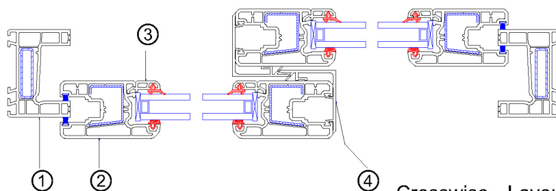
Crosswise Layout Drawing
