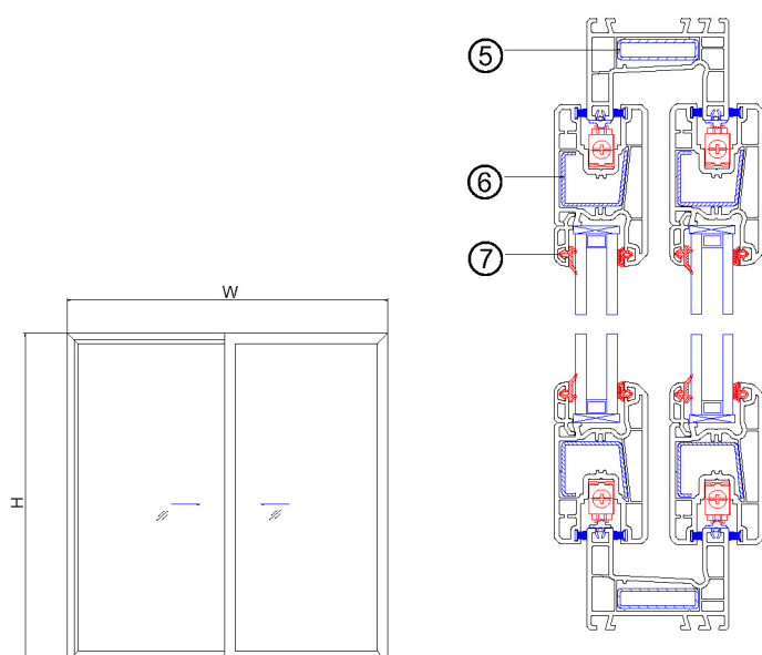
Vertical Layout Drawing
