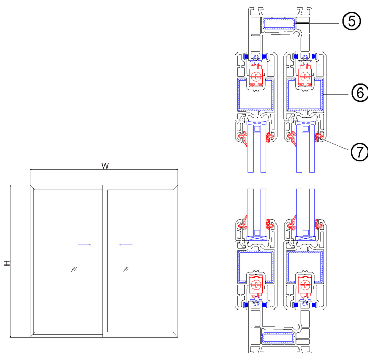
Vertical Layout Drawing
