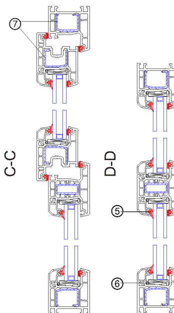
Vertical Assembly Drawing
