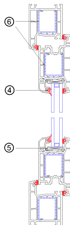
Vertical Assembly Drawing
