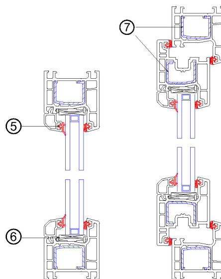
Vertical Assembly Drawing
