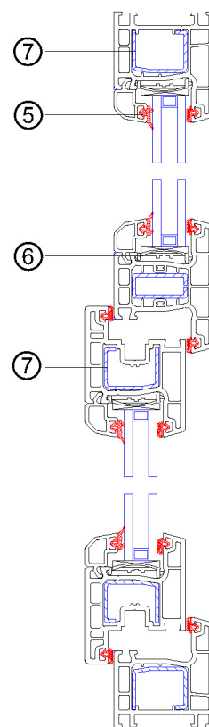
Vertical Assembly Drawing
