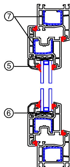
Vertical Assembly Drawing
